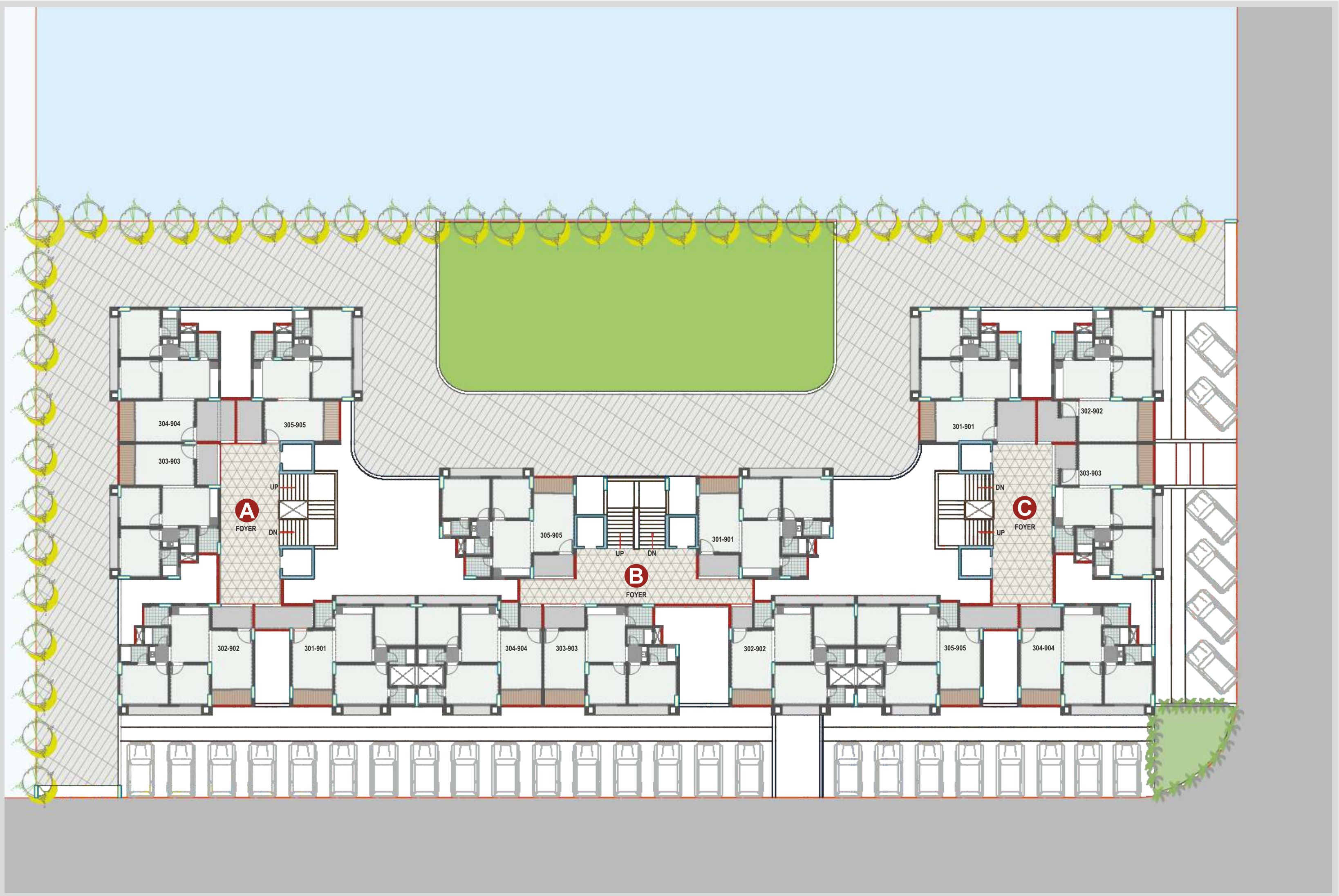
TYPICAL FLOOR PLAN | THIRD TO NINTH FLOOR
