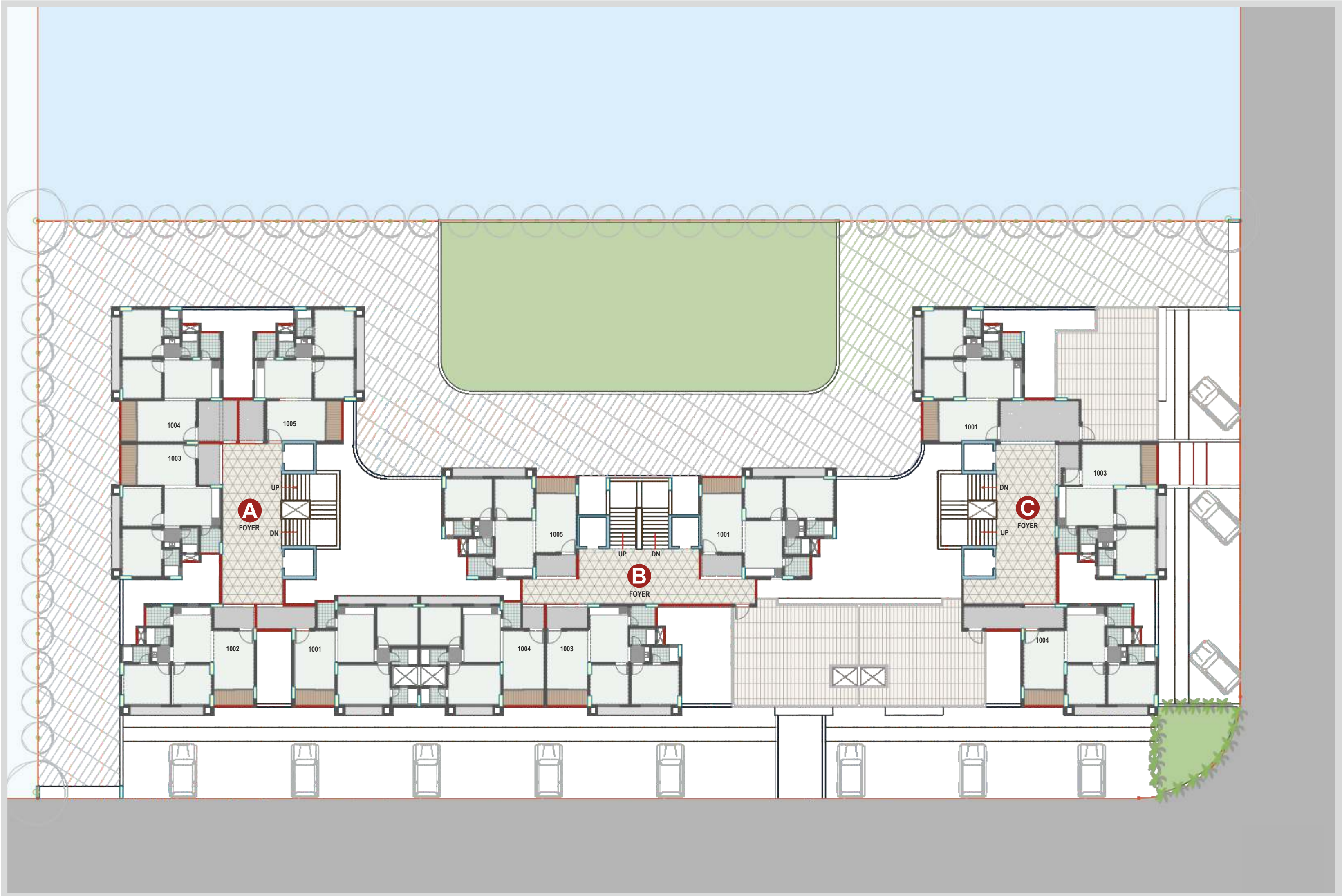
TENTH FLOOR PLAN
